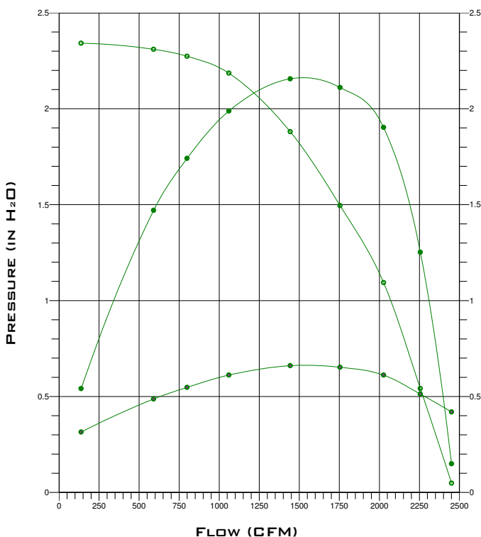
MODEL DSI, SIZE 140X PERFORMANCE CURVE
